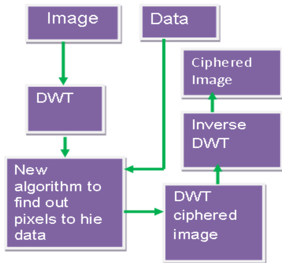
Figure 1: Proposed Data Hiding Method
