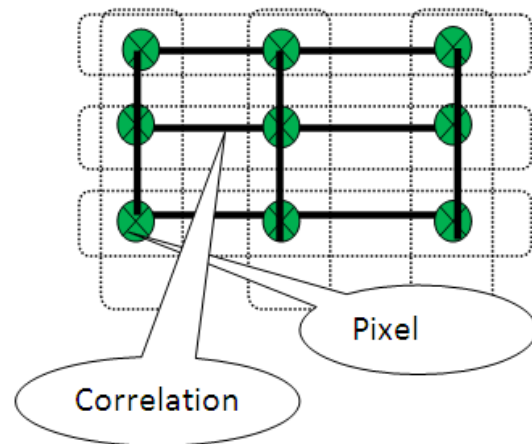
Figure 2: Correlation Approach
